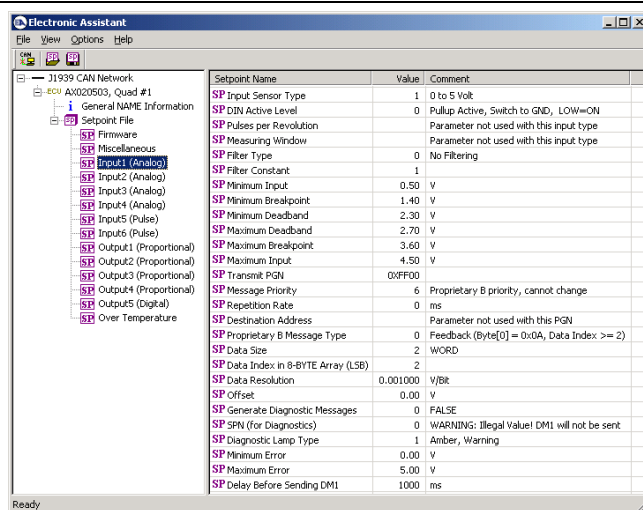
Figure 2.0 Configuration screen from the Electronic Assistant
