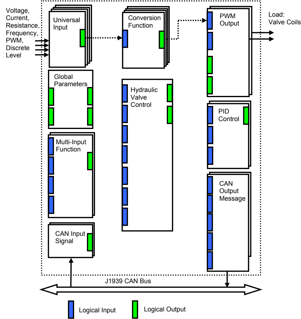
Fig. 1. Controller Architecture. As an example, one of universal inputs is connected to a conversion function and the conversion function is connected to a PWM output, providing a path for the input signal from input to output through the conversion function.
