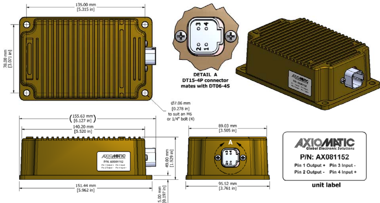
Figure 2.0 – Dimensional Drawing
