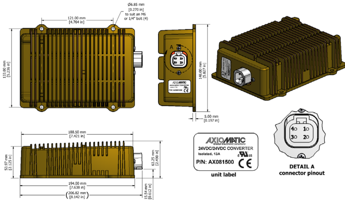
Figure 2.0 – Dimensional Drawing
