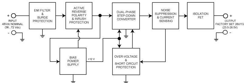
BLOCK DIAGRAM
