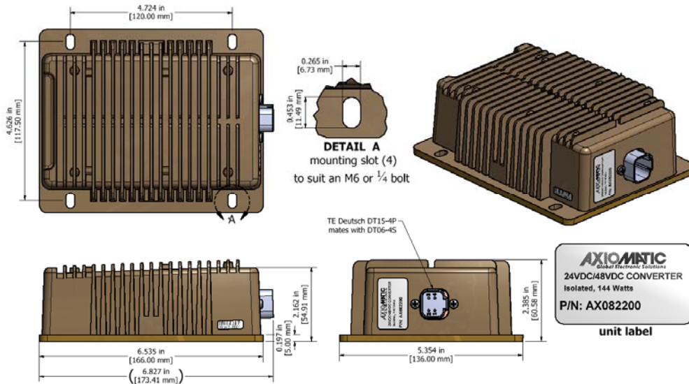
Figure 4.0. – Dimensional Drawing
