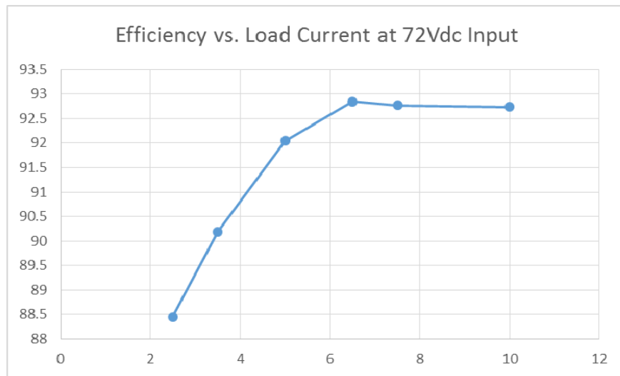
Figure 1.0 - Efficiency vs. Output Current at 72Vdc Input
