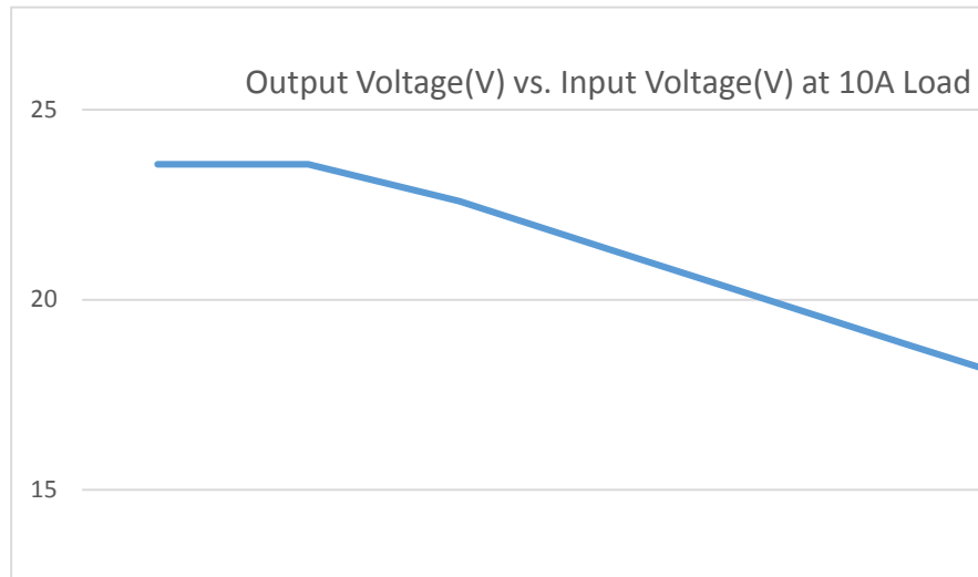
Figure 4.0 – Output Voltage vs. Input Voltage at 10A Load for Input less than 42Vdc
