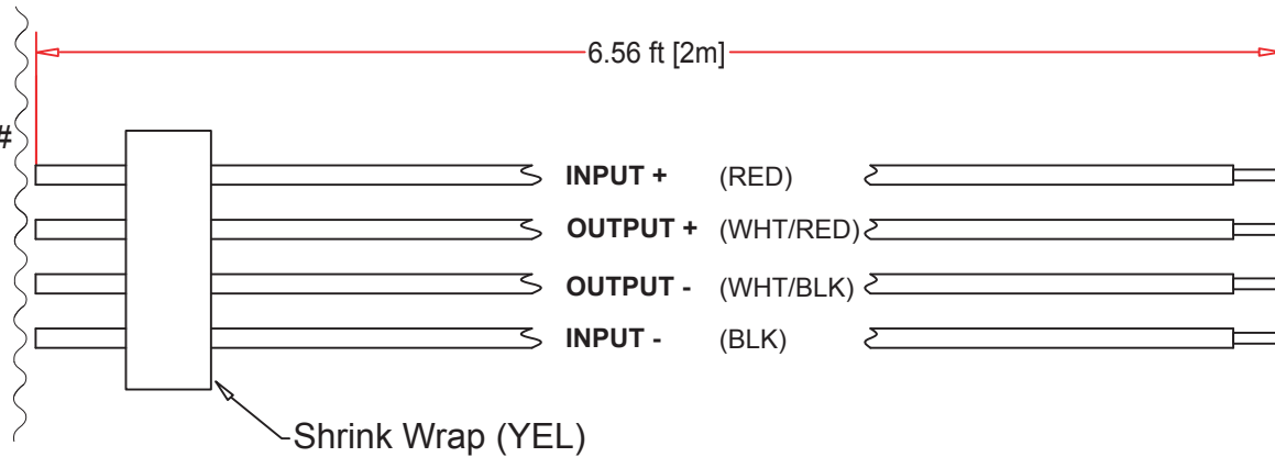
DTP06-4S Assembly
