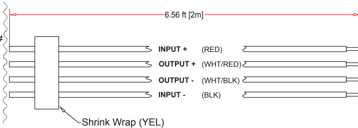
DTP06-4S Assembly
