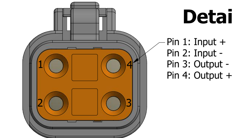
Detail A Deutsch DTP06-4S 4-Pin Plug Mates With DTP13-4P Receptacle
