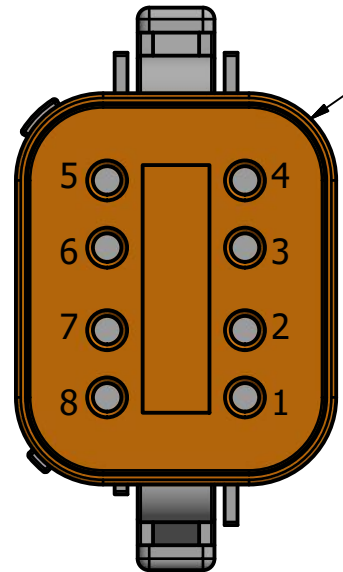
Detail A Deutsch DT06-08SA 8-Pin Plug Mates With DT13-08PA Connector
