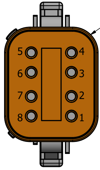
Detail A Deutsch DT06-8SA 8-Pin Plug Mates With DT13-8PA Connector
