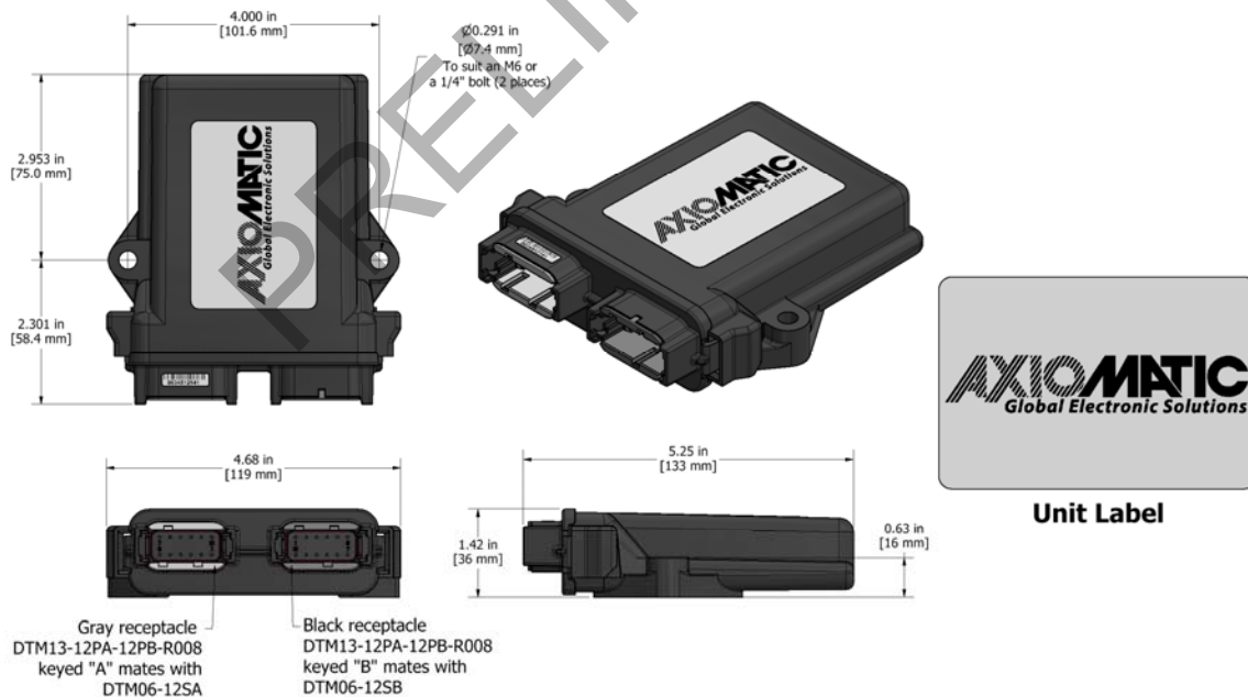
Figure 1.0 – Dimensional Drawing
