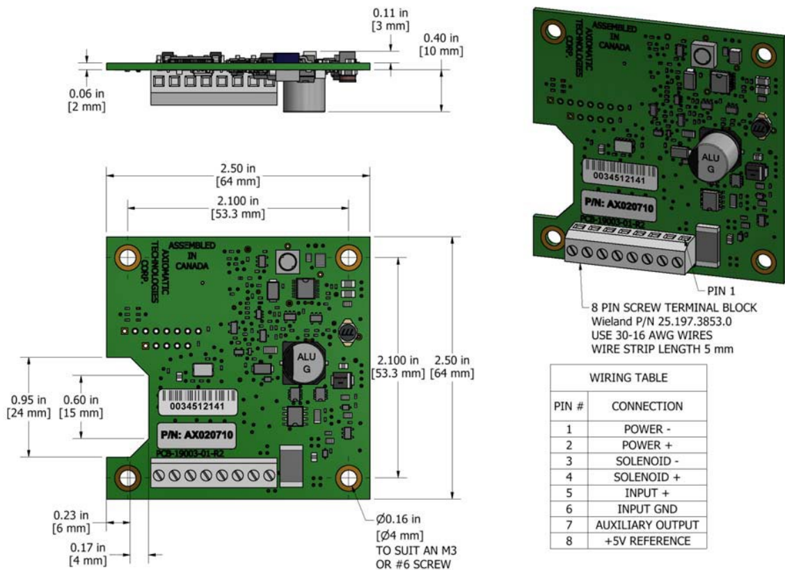
Figure 1.0. – Dimensional Drawing of AX0207X0
