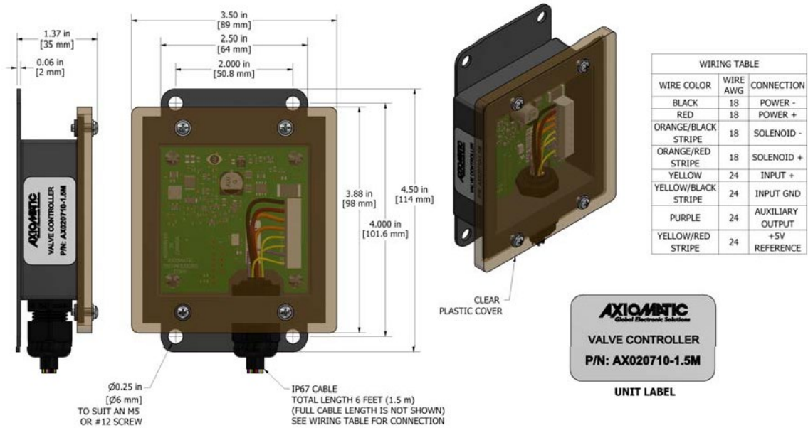
Figure 3.0 – Dimensional Drawing of AX0207X0-1.5M
