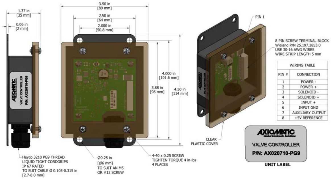
Figure 2.0 – Dimensional Drawing of AX0207X0-PG9
