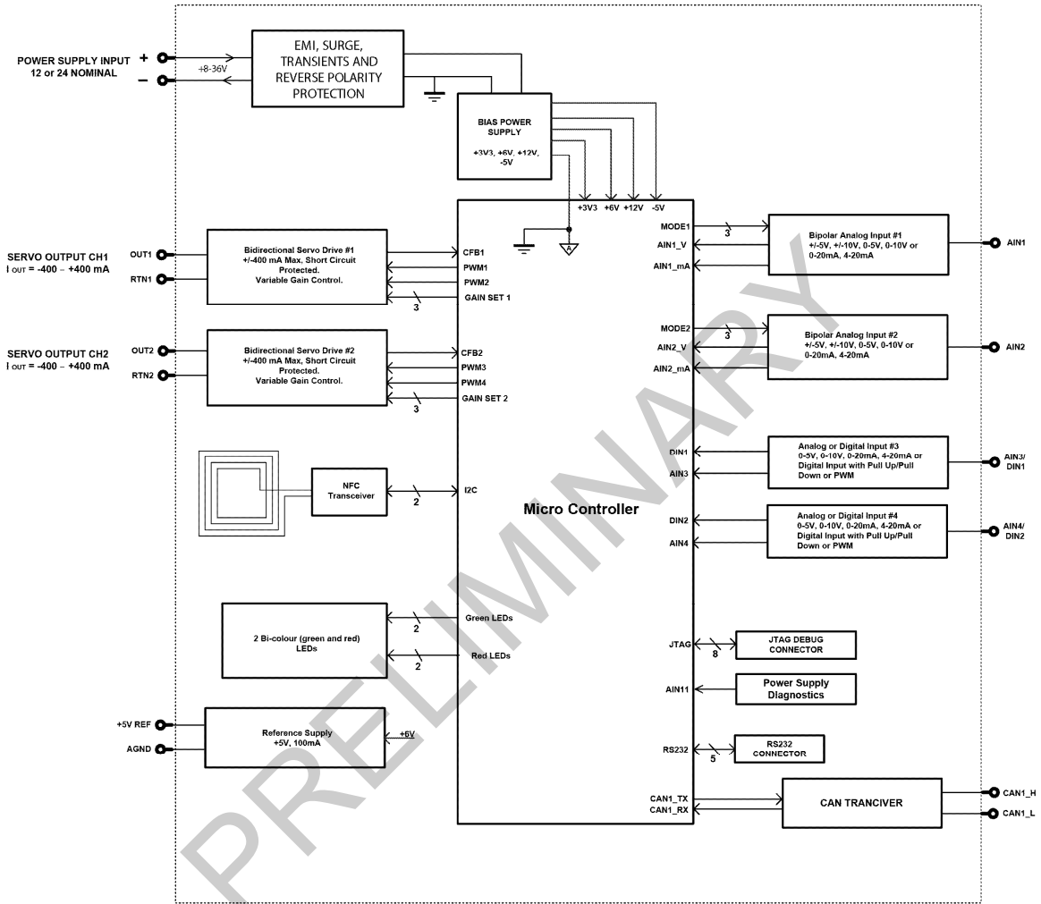
Figure 1.0 - Block Diagram
