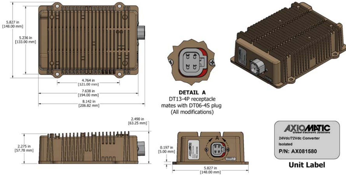
Figure 3.0. – Dimensional Drawing
