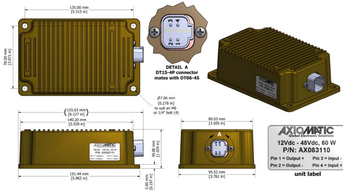
Figure 1.0 - Dimensional Drawing
