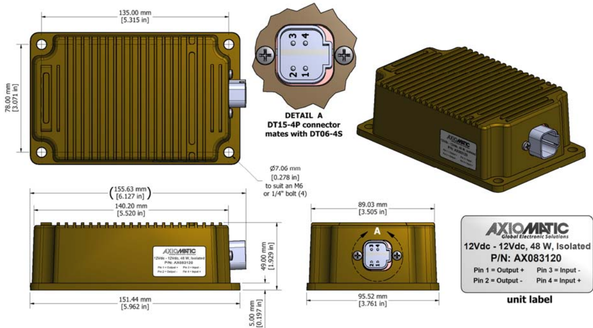
Figure 1.0 - Dimensional Drawing
