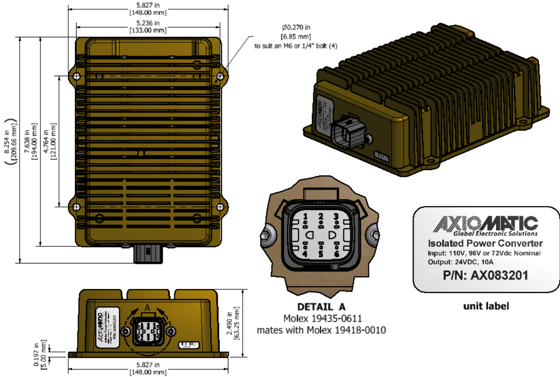
Figure 7.0 – Dimensional Drawing
