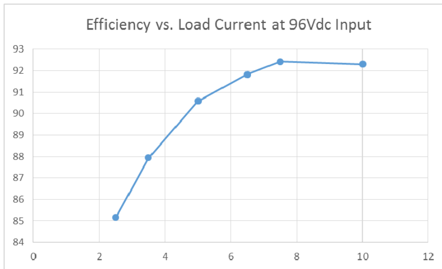
Figure 2.0 - Efficiency vs. Output Current at 96Vdc Input
