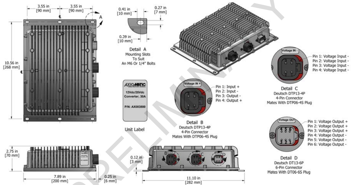
Figure 4. 0. – Dimensional Drawing
