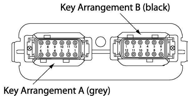
Figure 2.0 – Pin out
