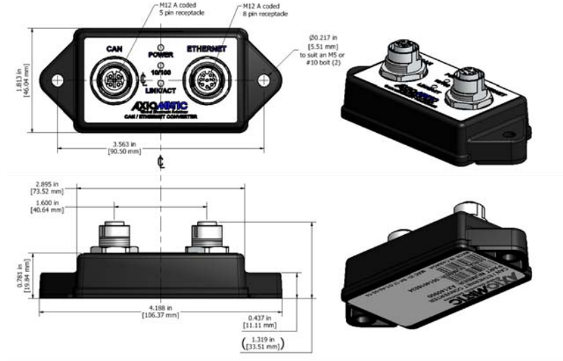
Figure 2.0. Dimensional Drawing
