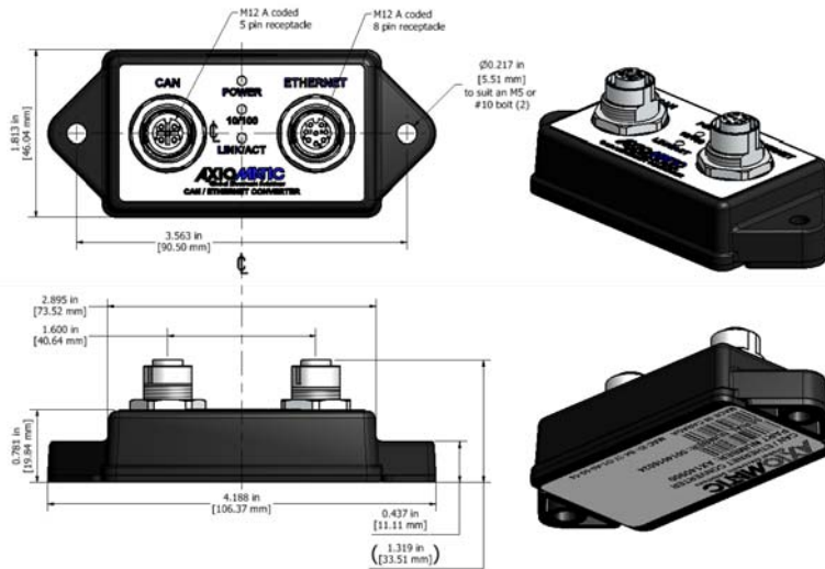
Figure 2.0. Dimensional Drawing
