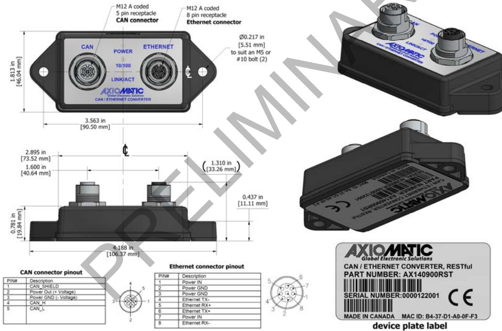
Figure 2.0. Dimensional Drawing
