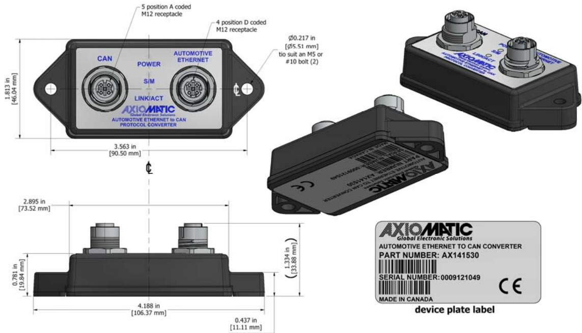
Figure 2.0. Dimensional Drawing
