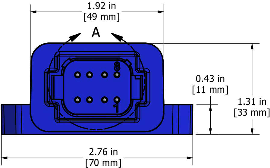
DETAIL A Molded in TE Deutsch receptacle, based on DT04-08PA, mates with DT06-08SA
