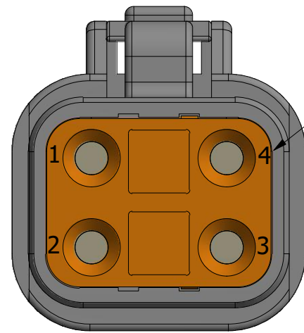
Detail A Deutsch DTP06-4S 4-Pin Plug Mates With DTP13-4P Receptacle
