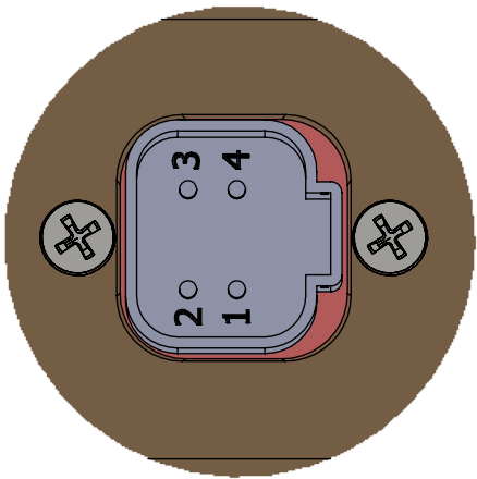
DETAIL C DT15-4P Connector mates with DT06-4S
