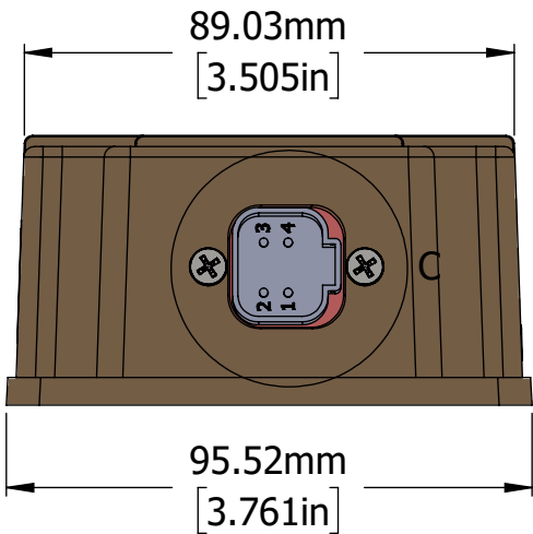
DETAIL C DT15-4P Connector mates with DT06-4S
