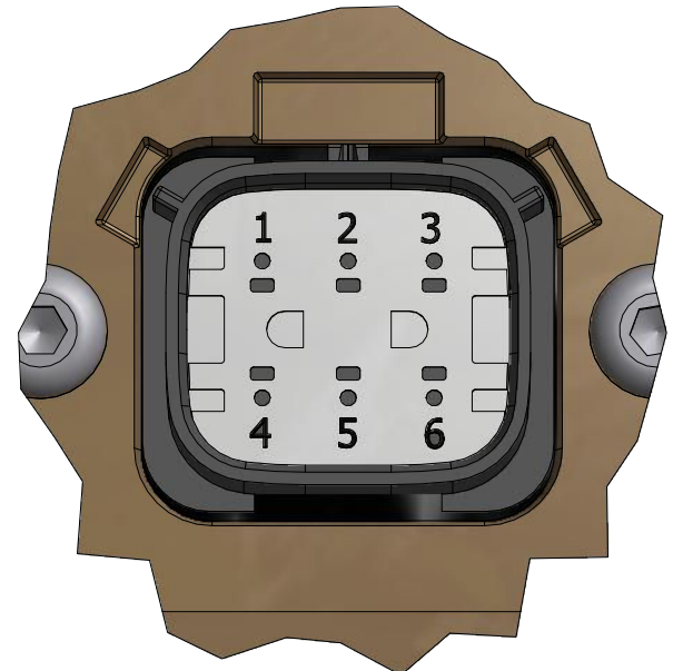
DETAIL A Molex 19435-0611 mates with Molex 19418-0010
