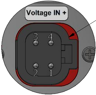
Detail B Deutsch DTP13-4P 4-Pin Connector Mates With DTP06-4S Plug
