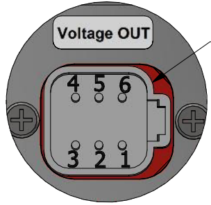
Detail D Deutsch DT13-6P 6-Pin Connector Mates With DT06-6S Plug
