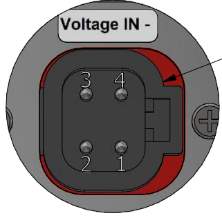
Detail C Deutsch DTP13-4P 4-Pin Connector Mates With DTP06-4S Plug
