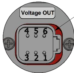
Detail D Deutsch DT13-6P 6-Pin Connector Mates With DT06-6S Plug
