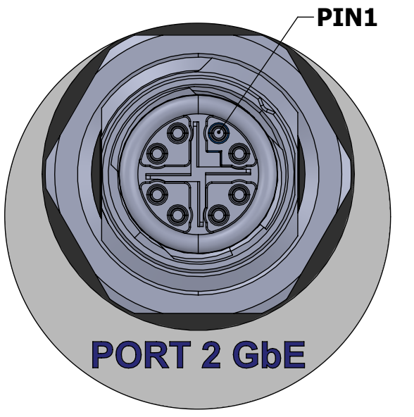
DETAIL C PORTS 2 / 3 / 4 Gigabit Ethernet X coded M12 female
