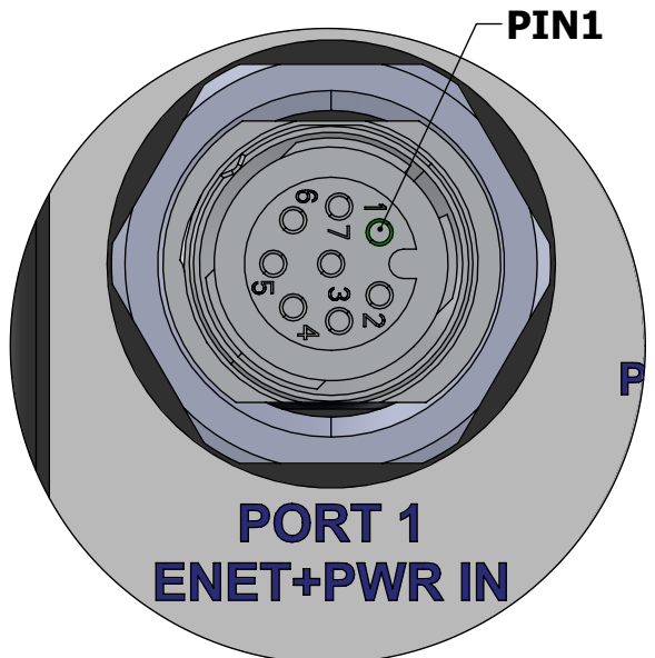
DETAIL B PORT 1 Ethernet and power in A coded M12 female
