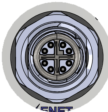
DETAIL A M12 X coded 8 position receptacle
