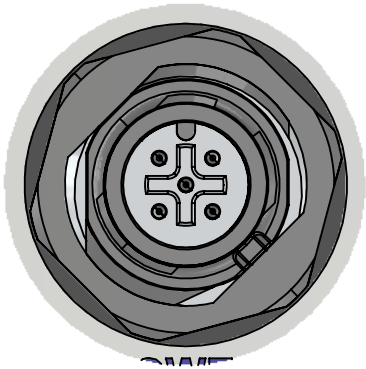
DETAIL C M12 A coded 5 position male plug
