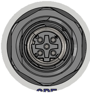
DETAIL B M12 D coded 4 position receptacle
