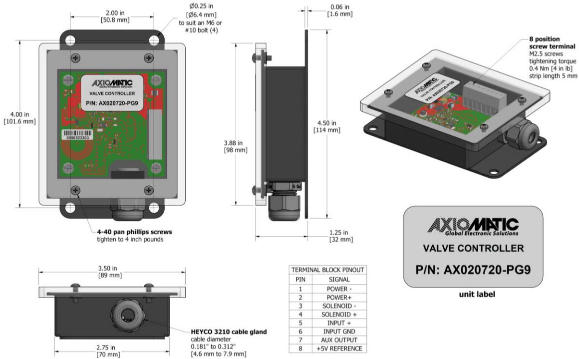
Figure 1.0 – Dimensional Drawing
