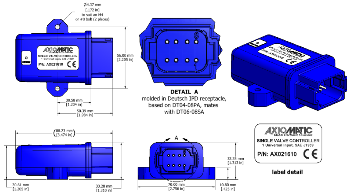
Figure 1.0. – Dimensional Drawing
