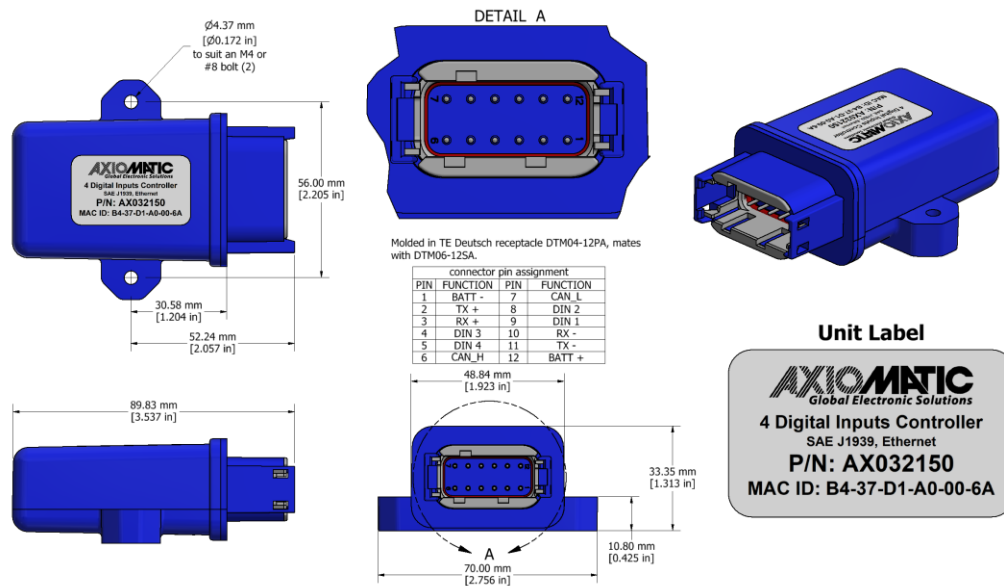
Figure 2.0 – Dimensional Drawing of AX032150
