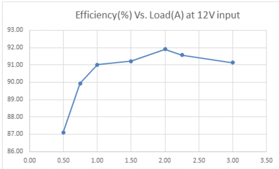
Figure 1.0 - Efficiency vs. Output Current at 12Vdc Input
