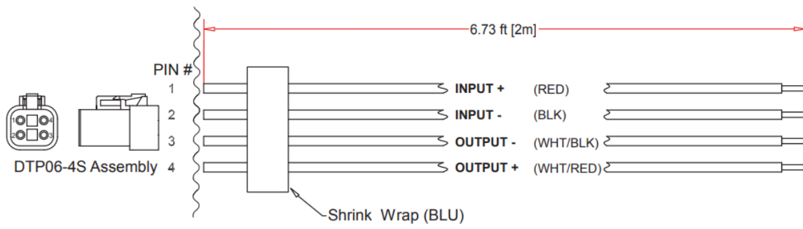
Figure 3.0. – Wire Harness AX070103
