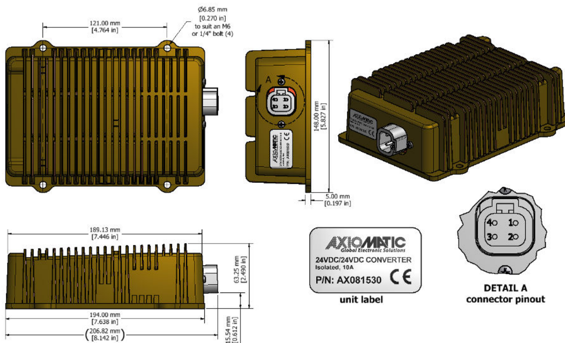
Figure 4. 0. – Dimensional Drawing
