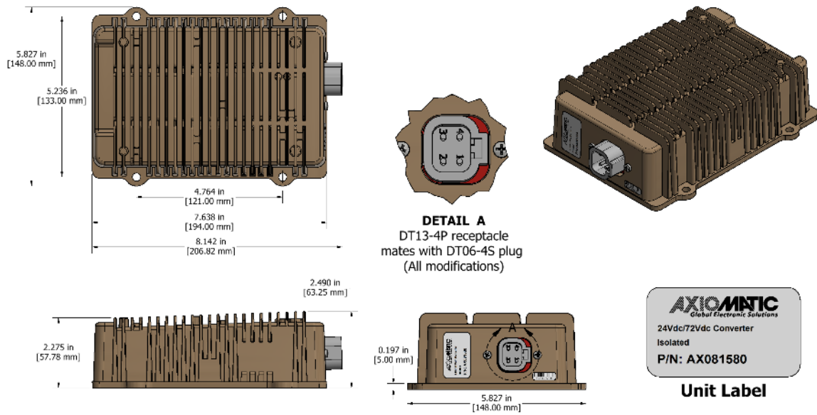
Figure 3.0. – Dimensional Drawing
