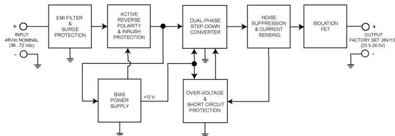
BLOCK DIAGRAM
