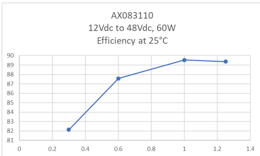
Figure 2.0 - Efficiency (%) vs. Output (A)
