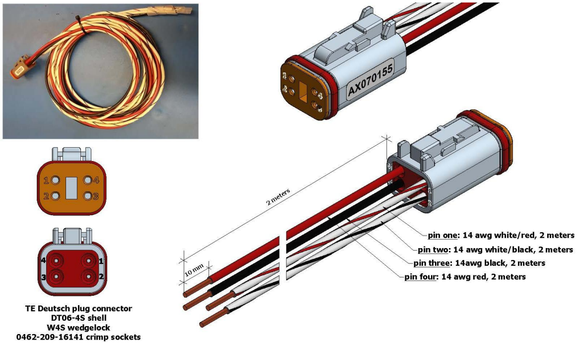
Figure 3.0 – Dimensional Drawing of AX070155 Wire Harness
