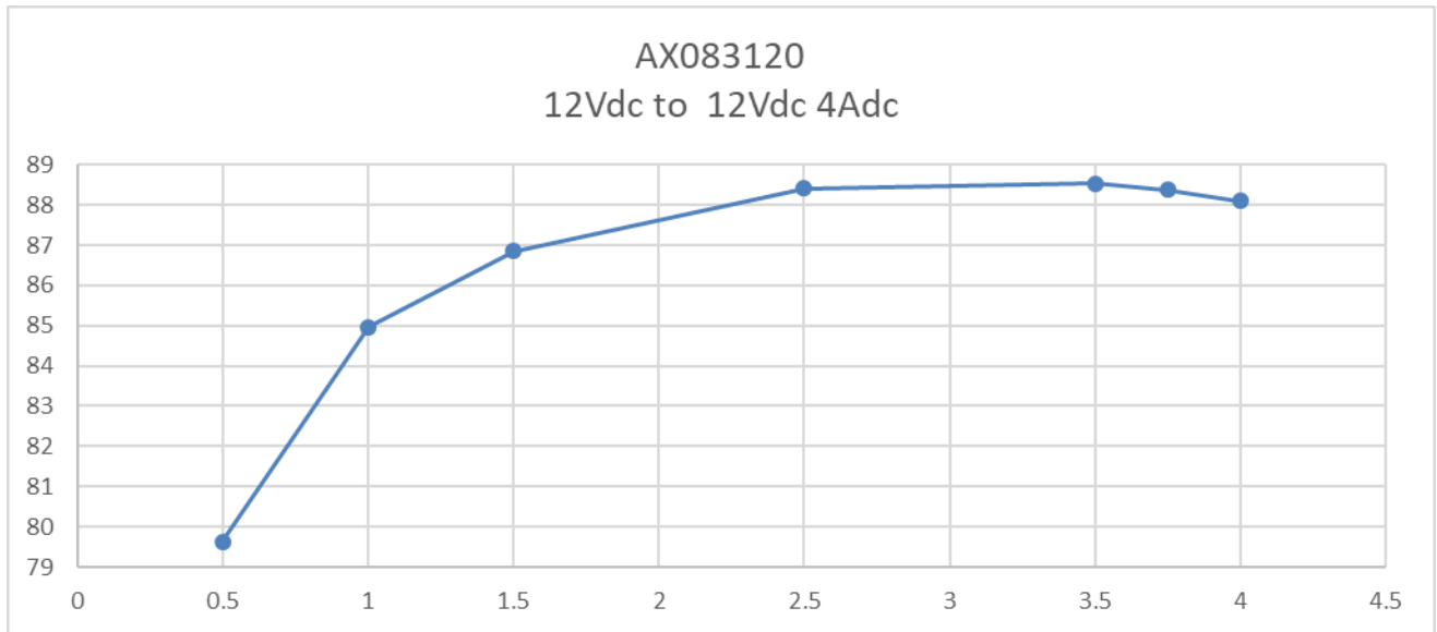
Figure 2.0 - Efficiency (%) vs. Output (A) – 4A model shown – 5A model not shown
