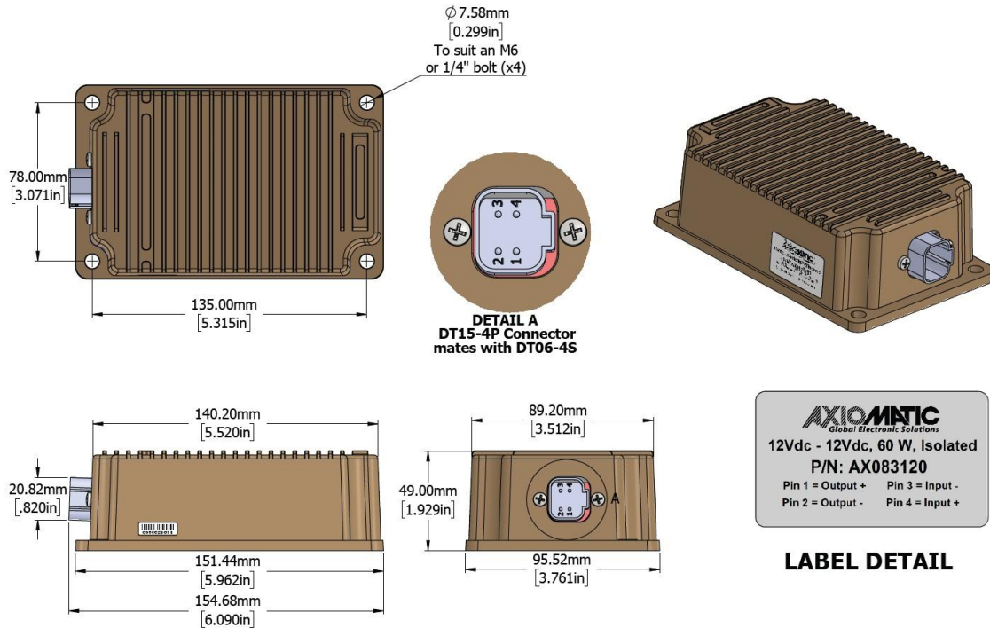
Figure 1.0 - Dimensional Drawing of AX083120 Converter
