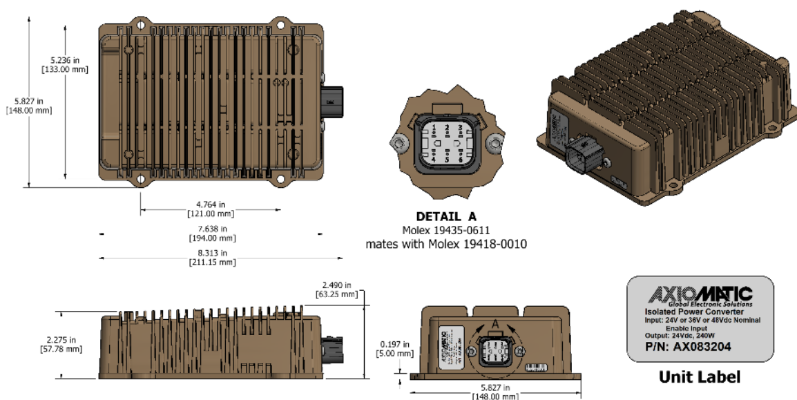
Figure 3.0 – Dimensional Drawing
