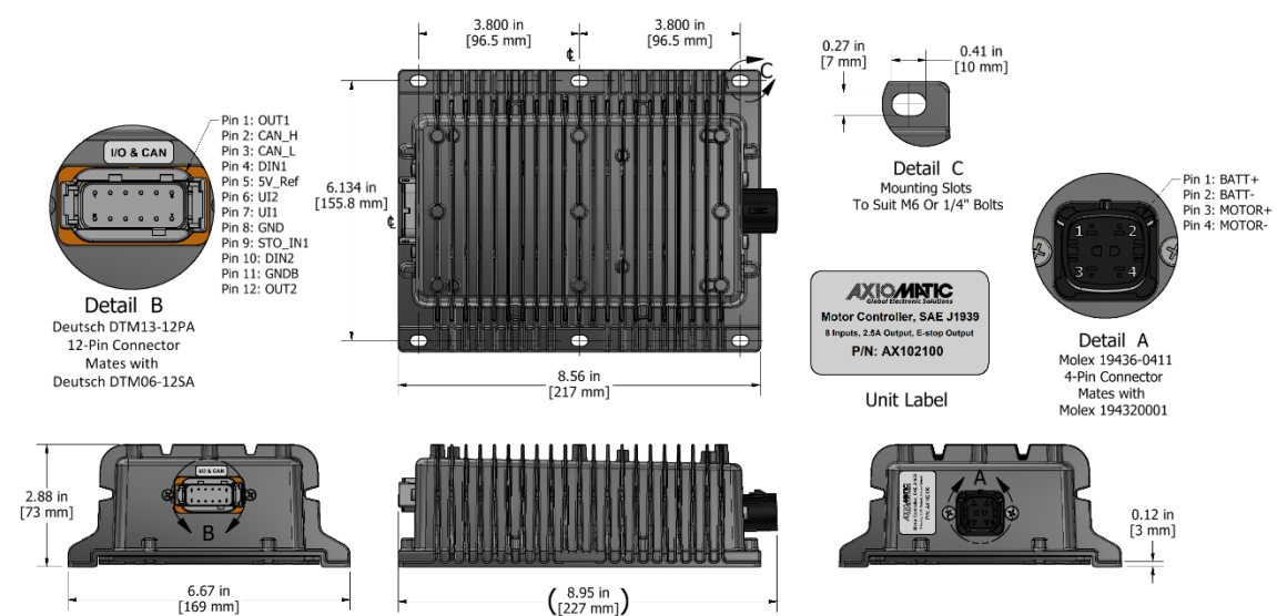
Figure 3 - Dimensional Drawing
