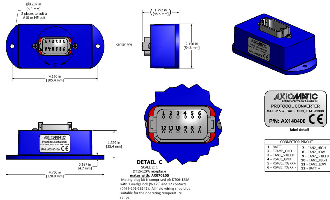
Figure 1.0 – Dimensional Drawing for AX140400
