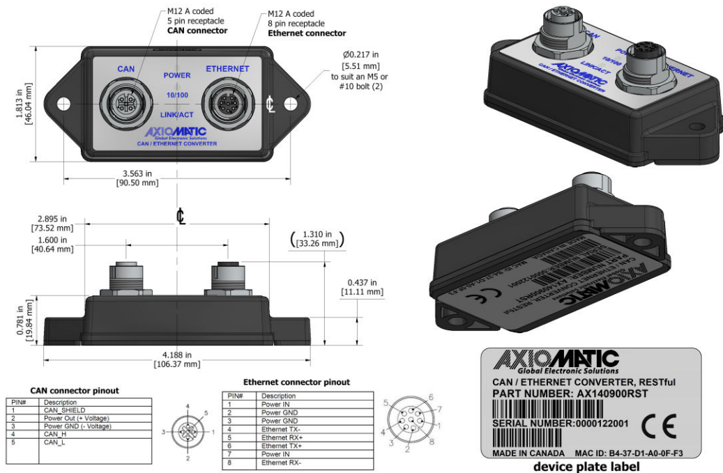
Figure 2.0. Dimensional Drawing
