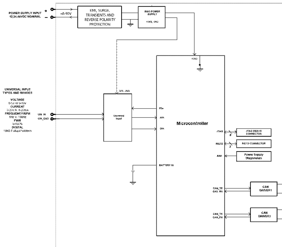
Figure 1.0 – Block Diagram
