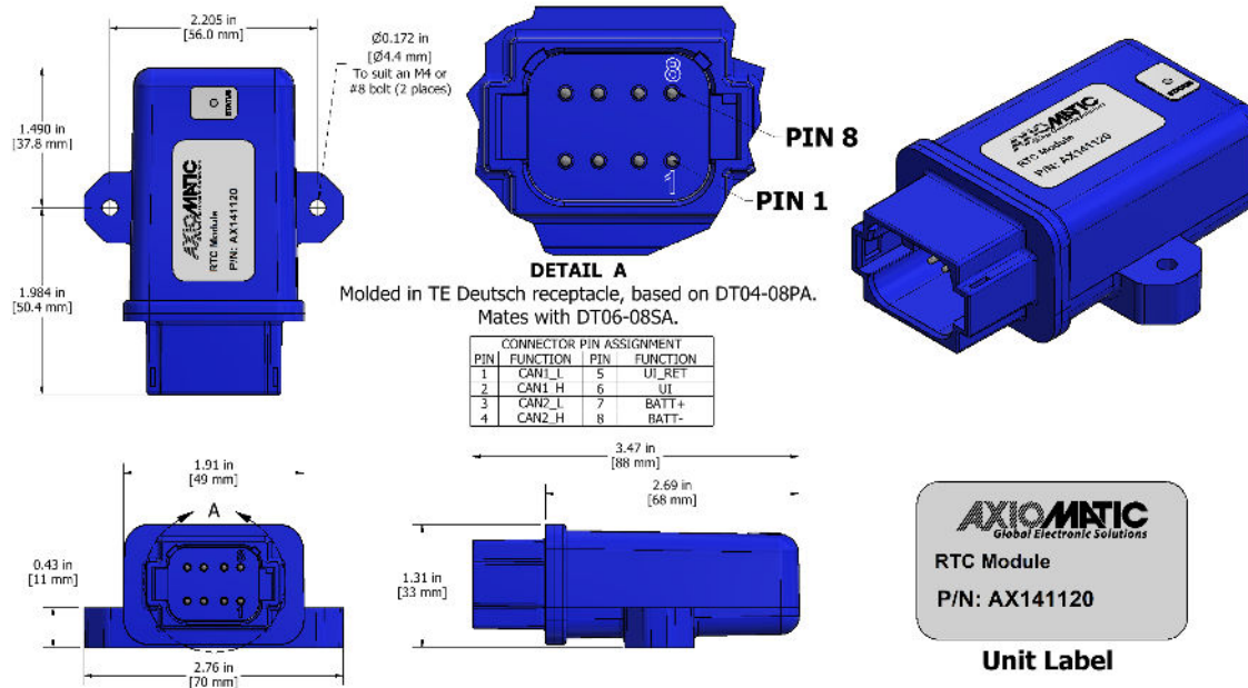
Figure 2.0 – Dimensional Drawing
