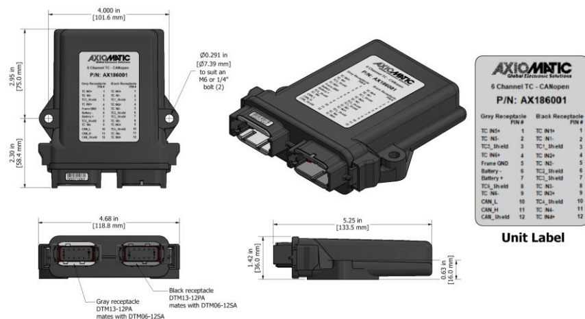
Figure 1.0 - Dimensional Drawing
