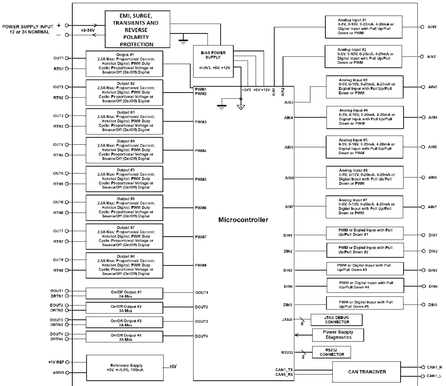
Figure 1A – Hardware Functional Block Diagram
