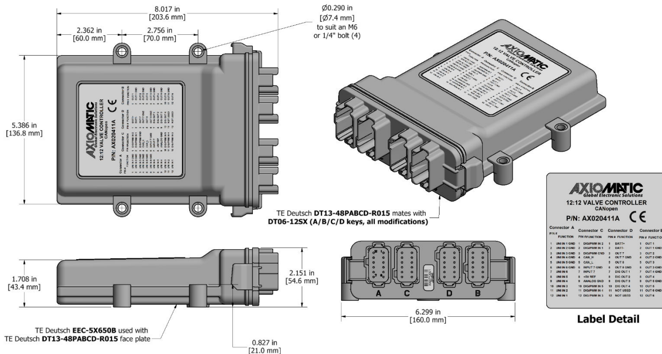
Figure 22 – Housing Dimensions
