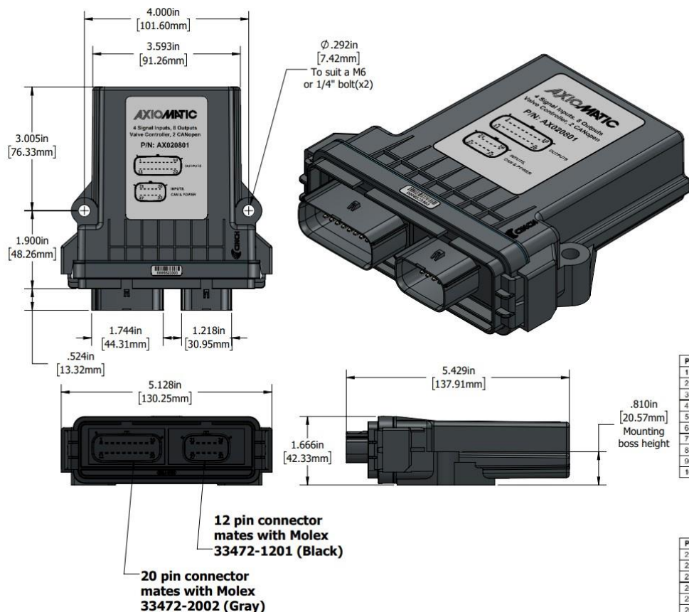
Figure 16 – Housing Dimensions
