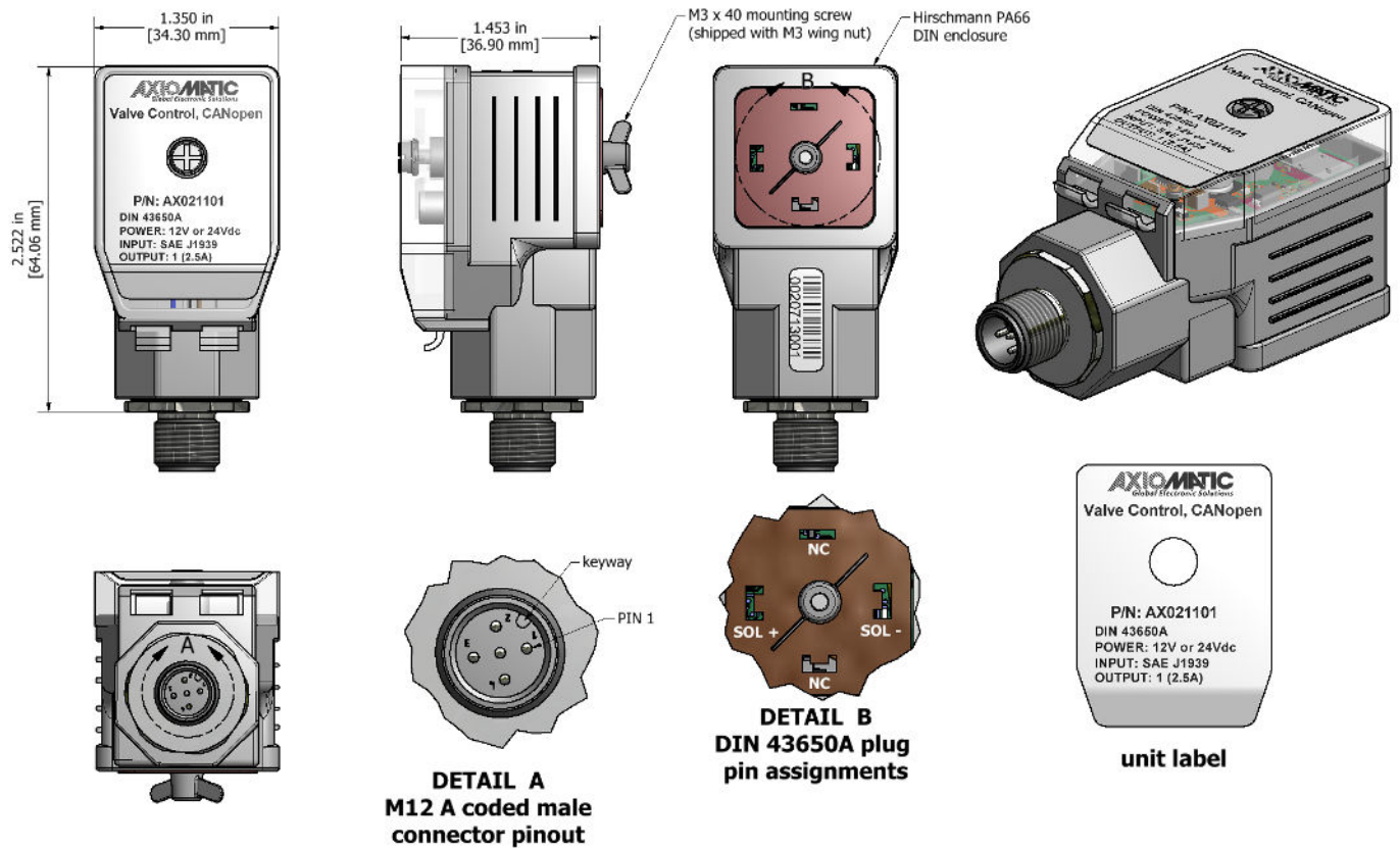
Figure 16 – Dimension Drawing
